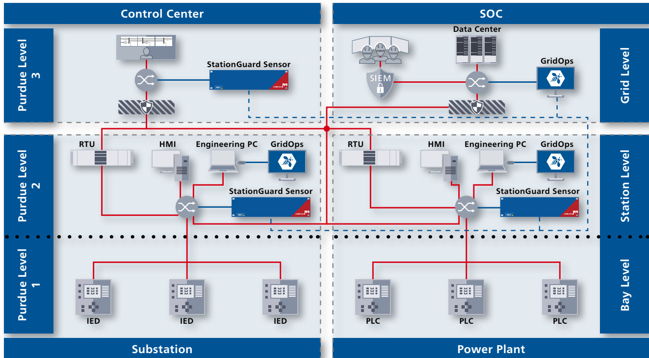
StationGuard Deployment Diagram
